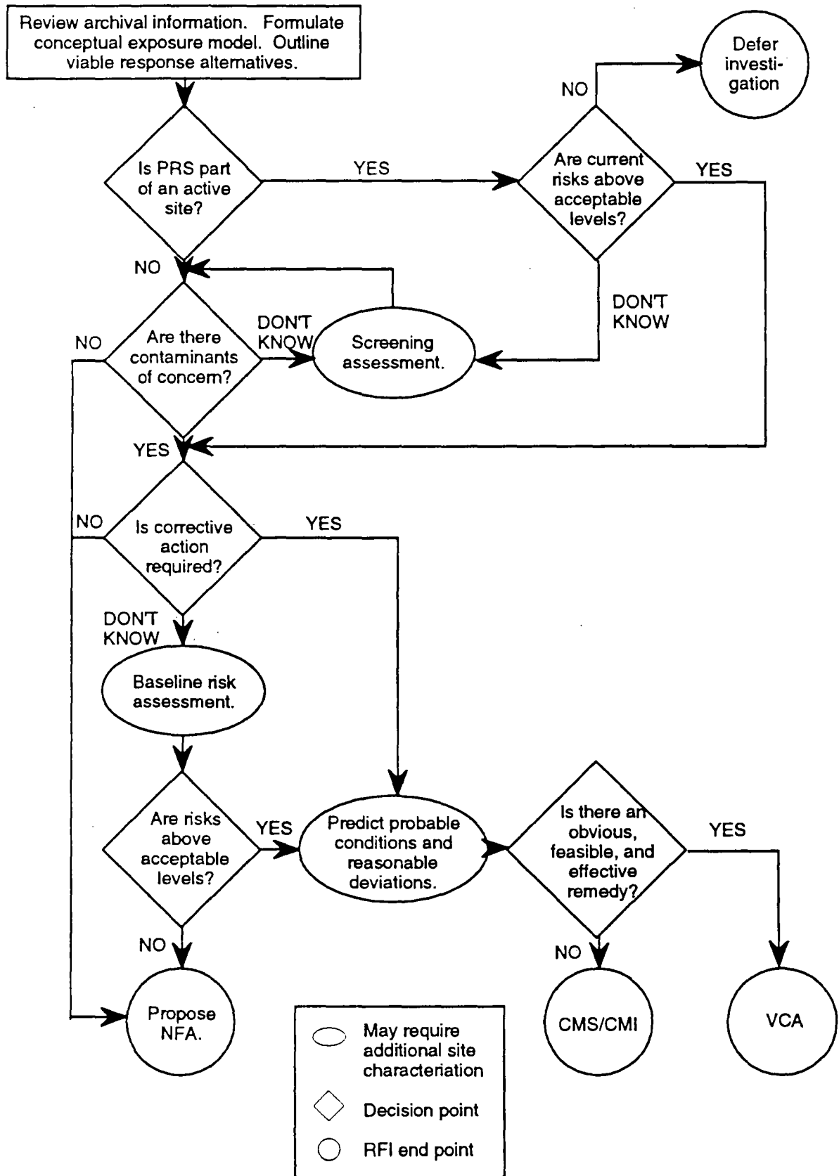
Figure 4-1. Decision flow during the RFI.
