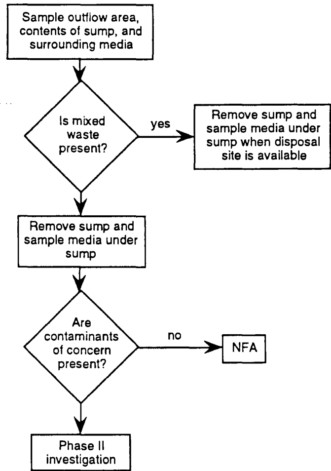
Figure 5-11. Logic flow diagram for Phase I sampling of inactive sump SWMUs.
