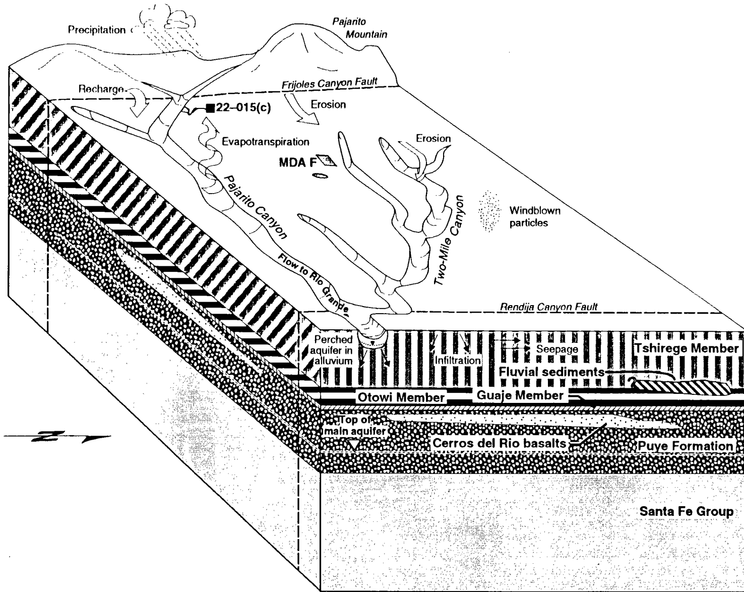
Figure 3-8. Conceptual hydrogeologic model of OU 1111.
