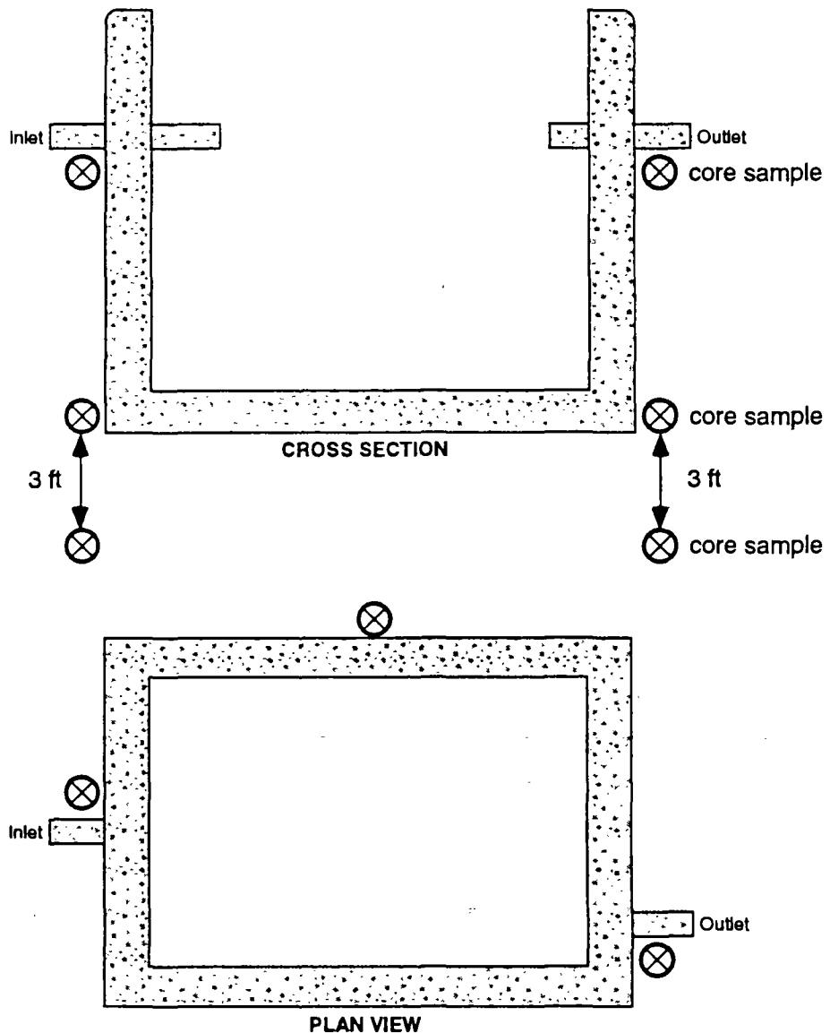
Figure 5-29. Diagram of approximate locations of cores around a septic tank. At least eight additional sampling locations will be sited upon removal of inactive septic tanks.
