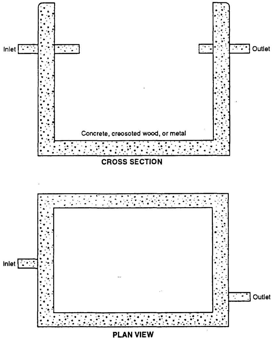
Figure 5-22. Diagram of a typical septic tank.
