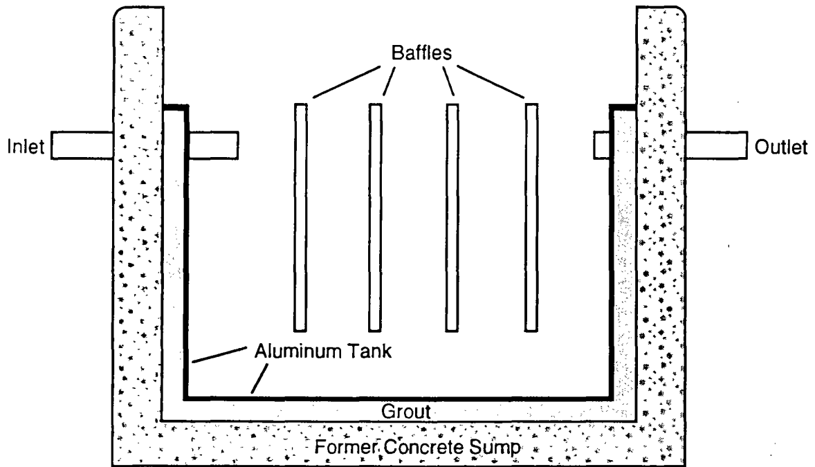
CROSS SECTION
