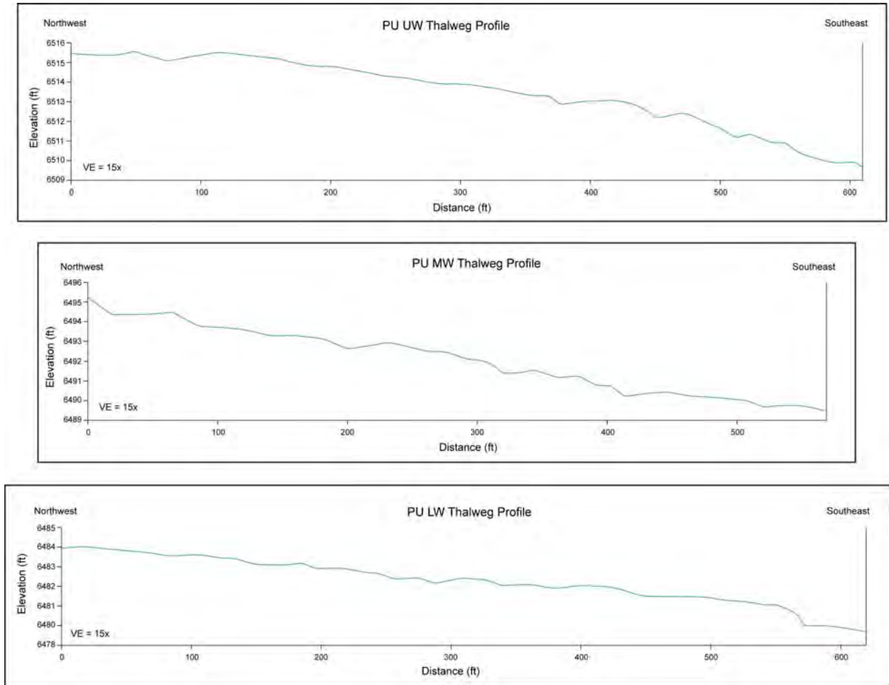
Figure 10 Thalweg profiles in the upper Pueblo Canyon willow-planting area
