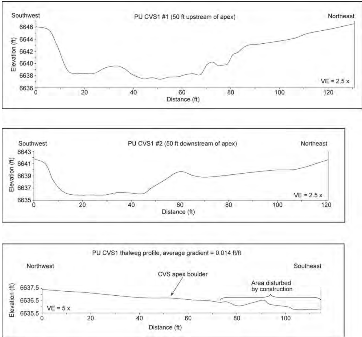
Figure 3 Cross sections and thalweg profile at upper CVS in Pueblo Canyon
