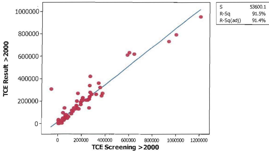
Figure 6. Correlation for TCE Results > Henry's Law Screen
