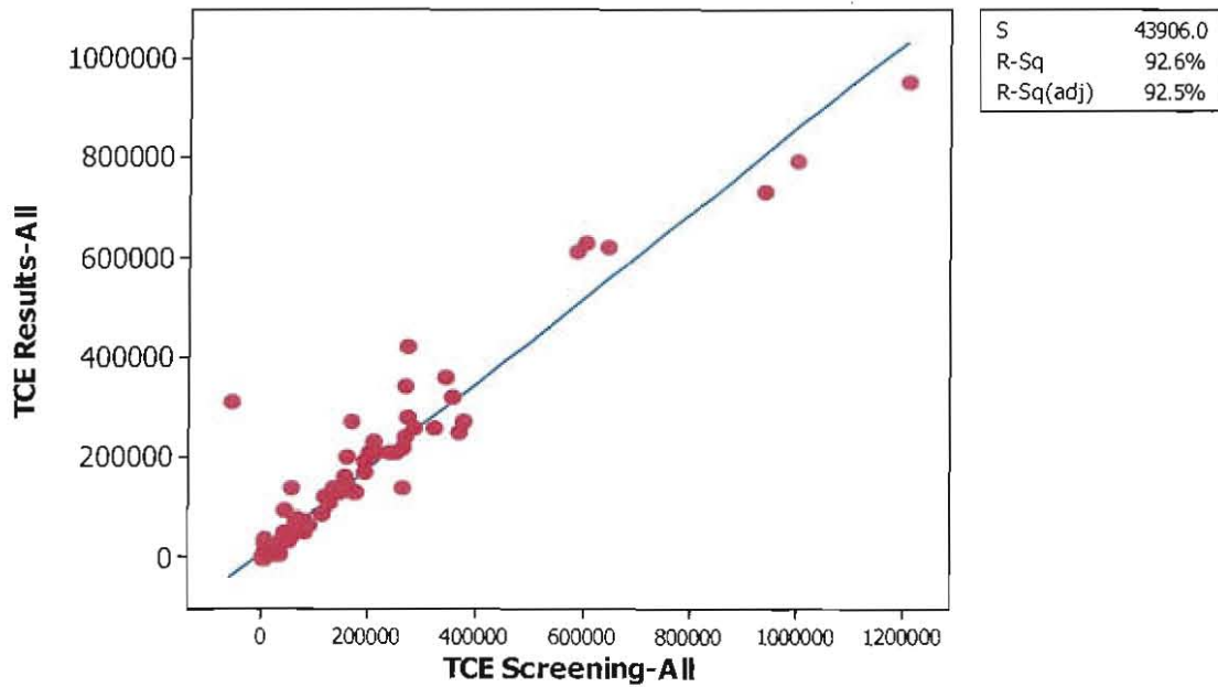
Figure 4. Correlation for TCE (All Data)
