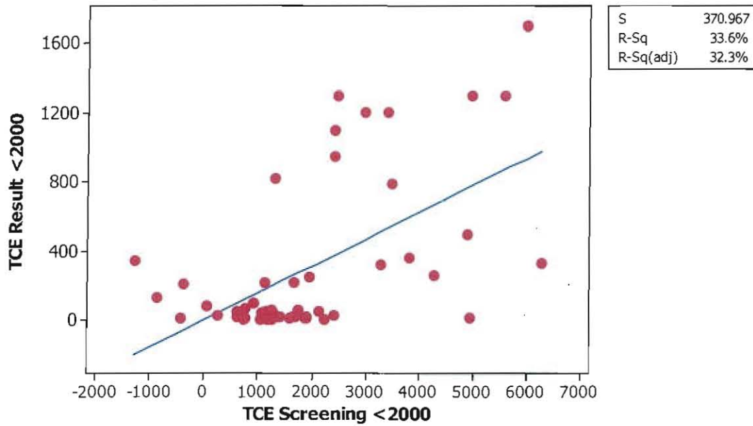
Figure 5. Correlation for TCE Results < Henry's Law Screen
