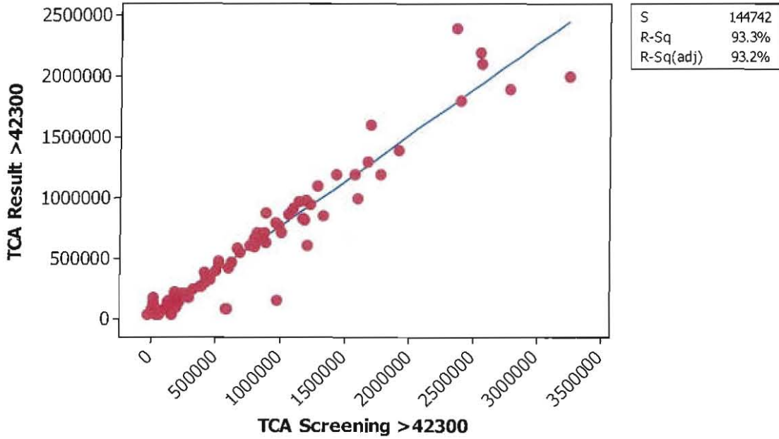
Figure 3. Correlation for TCA Results > Henry's Law Screen
