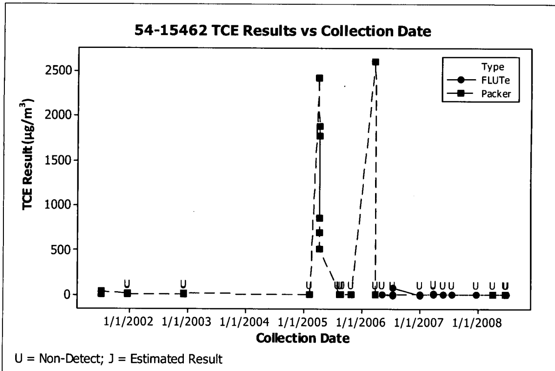
Figure 4.0-3 TCE results for all samples collected using the packer and FLUTe sampling systems in borehole location 54-15462 since 2001
