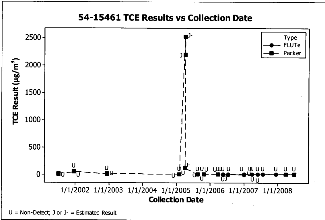
Figure 4.0-2 TCE results for all samples collected from using the packer and FLUTe sampling systems in borehole location 54-15461 since 2001
