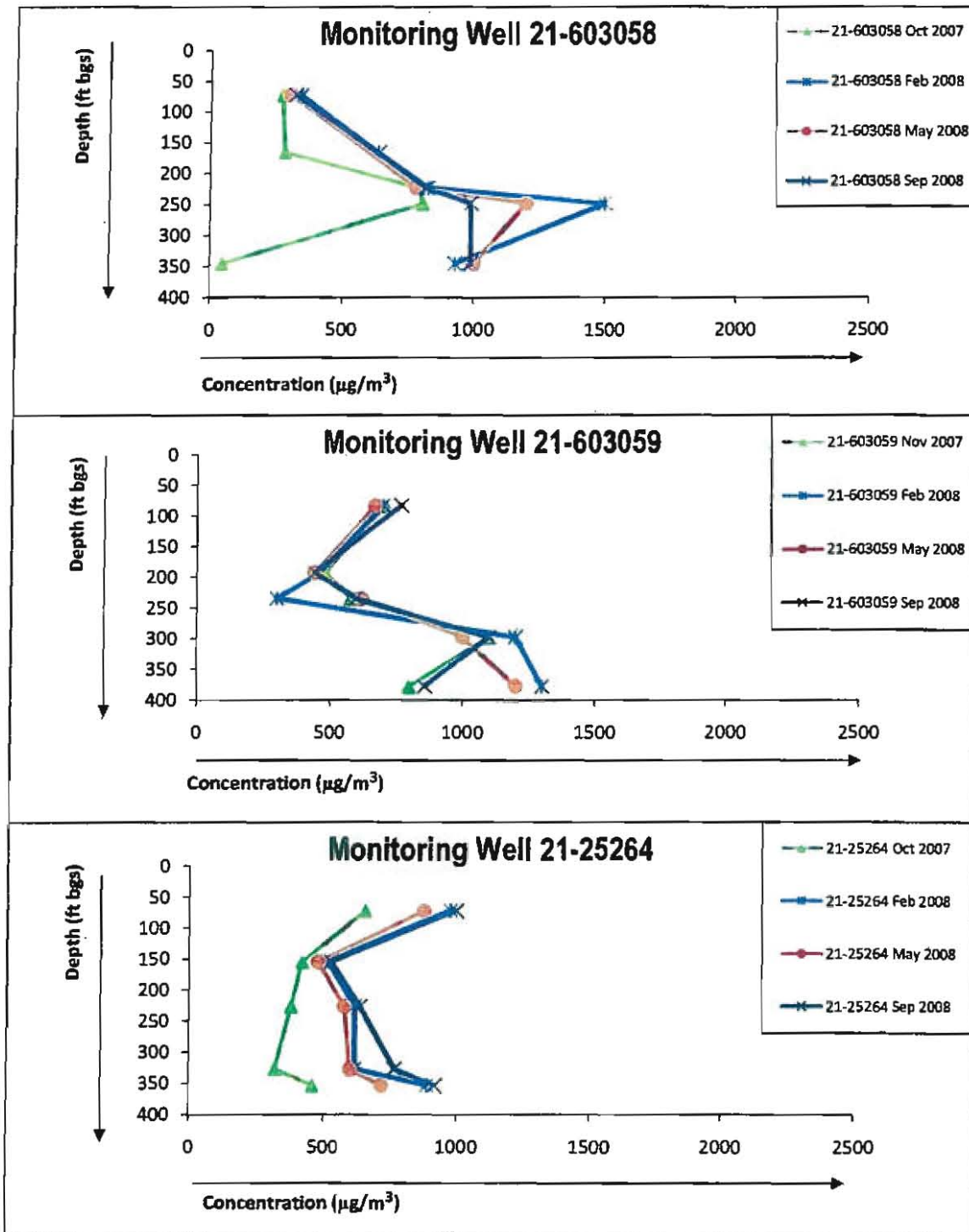
Vertical profile of TCE in pore gas, Monitoring Wells 21-603058, 21-603059, and 21-25264, First-Fourth Quarter, October 2007-September 2008.
