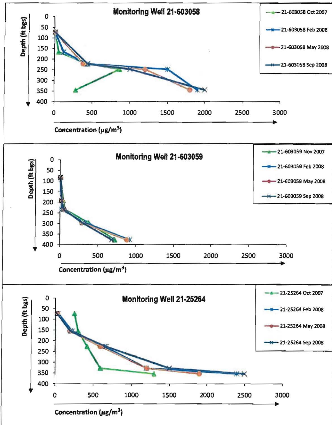
Vertical profile of methylene chloride in pore gas, Monitoring Wells 21-603058, 21-603059, and 21-25264, First–Fourth Quarter, October 2007–September 2008.
