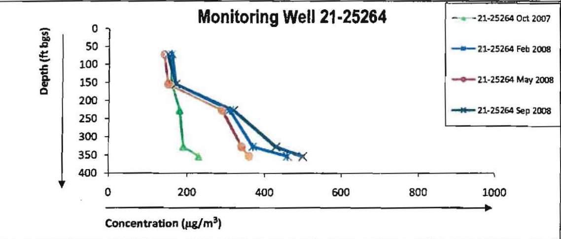
Vertical profile of carbon tetrachloride in pore gas, Monitoring Wells 21-603058, 21-603059, and 21-25264, First–Fourth Quarter, October 2007–September 2008.
