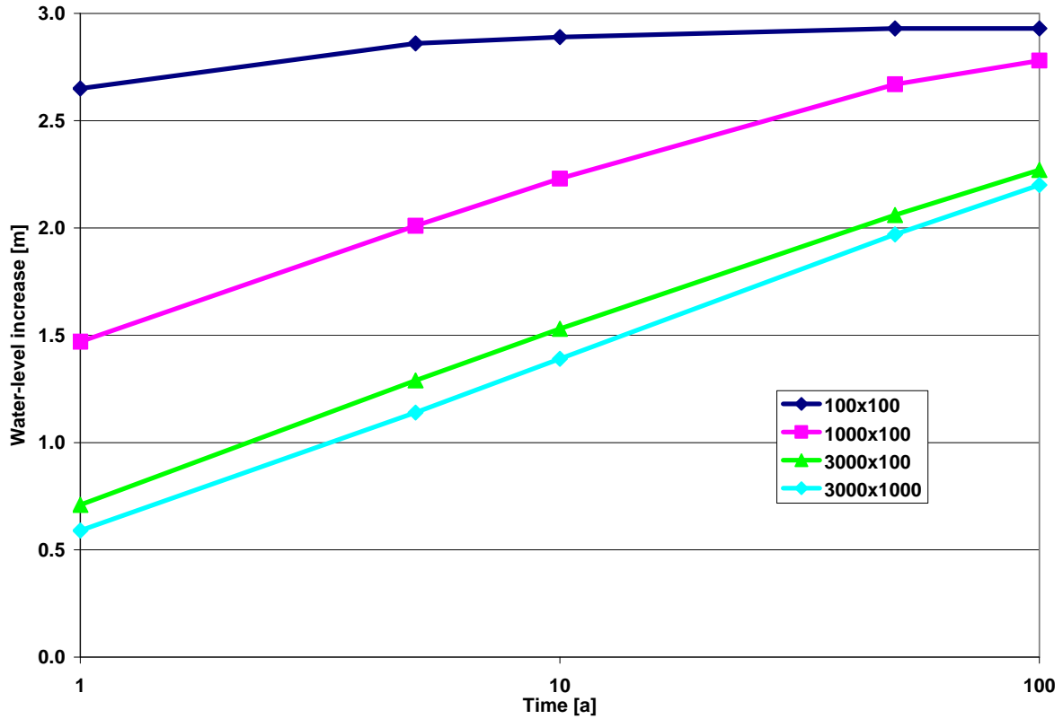
Figure I-1 Maximum increase of water levels within a mound (at the center of the mound) caused by a constant recharge of 1041 m 3 /d (275,000 gal./d) distributed over four different recharge areas ( A \times B ). The other parameters are k = 20 m/d, S = 0.1 , h_i = 10 m.
