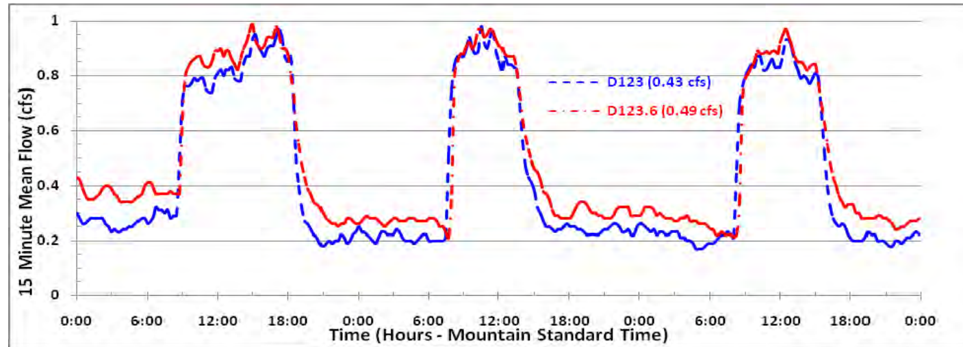
Figure C-1.0-2 Hydrographs from gaging stations D123 and D123.6 from April 21 to April 23, 2008, with time of D123.6 hydrograph shifted by 1.5 hr to better show relationship with D123; average daily discharge at gages shown in parentheses; average discharge from NPDES outfalls = 0.55 cfs for this period
