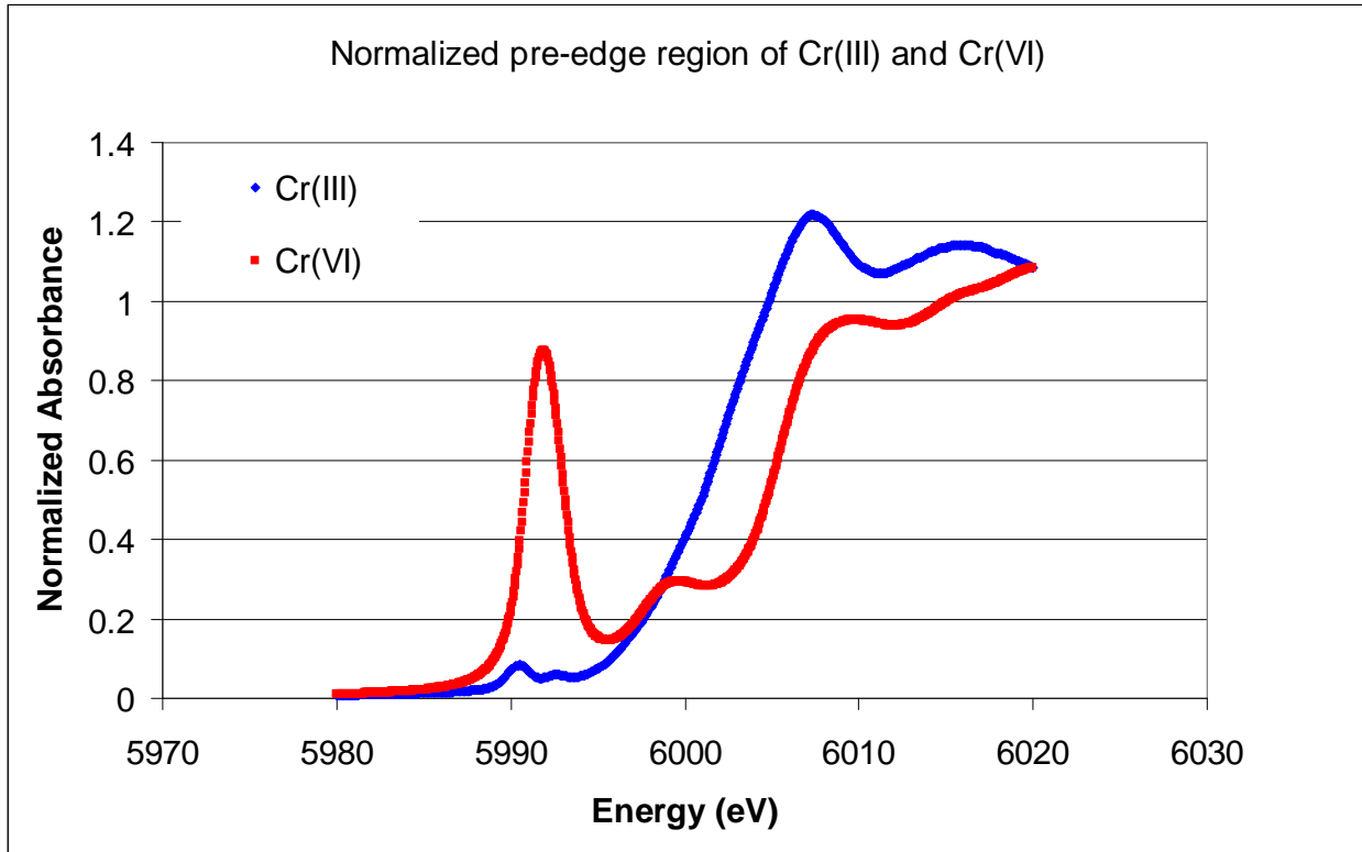
Figure K-3.1-1 Normalized pre-edge region of Cr 2 O 3 and K 2 CrO 4
