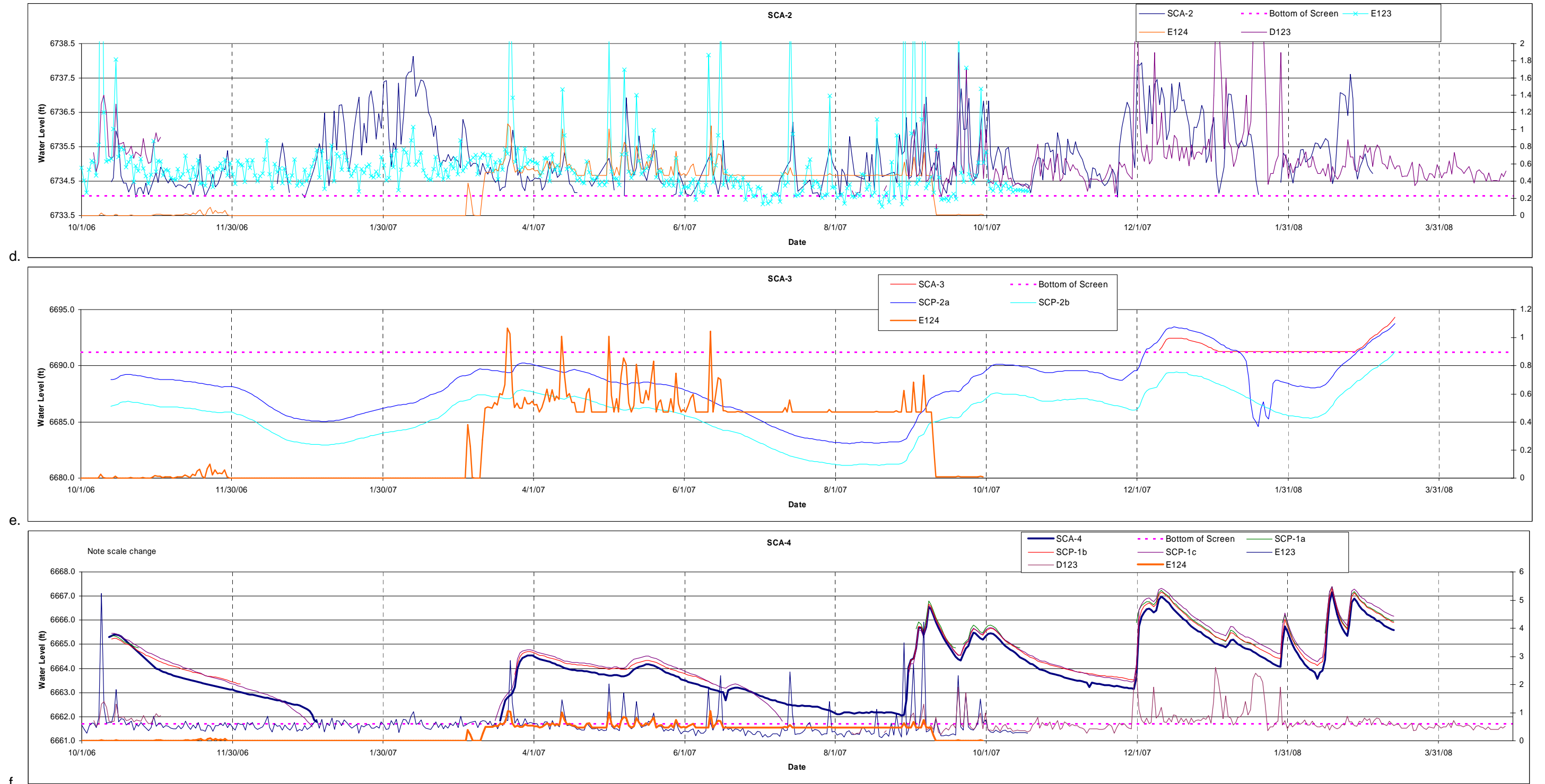
Figure C-2.0-1 (continued) Mean-daily alluvial water levels measured in wells SCA-1, SCA-2, SCA-3, and SCA-4 and piezometers SCP-1a,b,c and SCP-2a,b for the period of record, October 2006 to April 2008. Also shown are data for Sandia Canyon outfall volumes and stream gage, and TA-06 precipitation and temperature records
