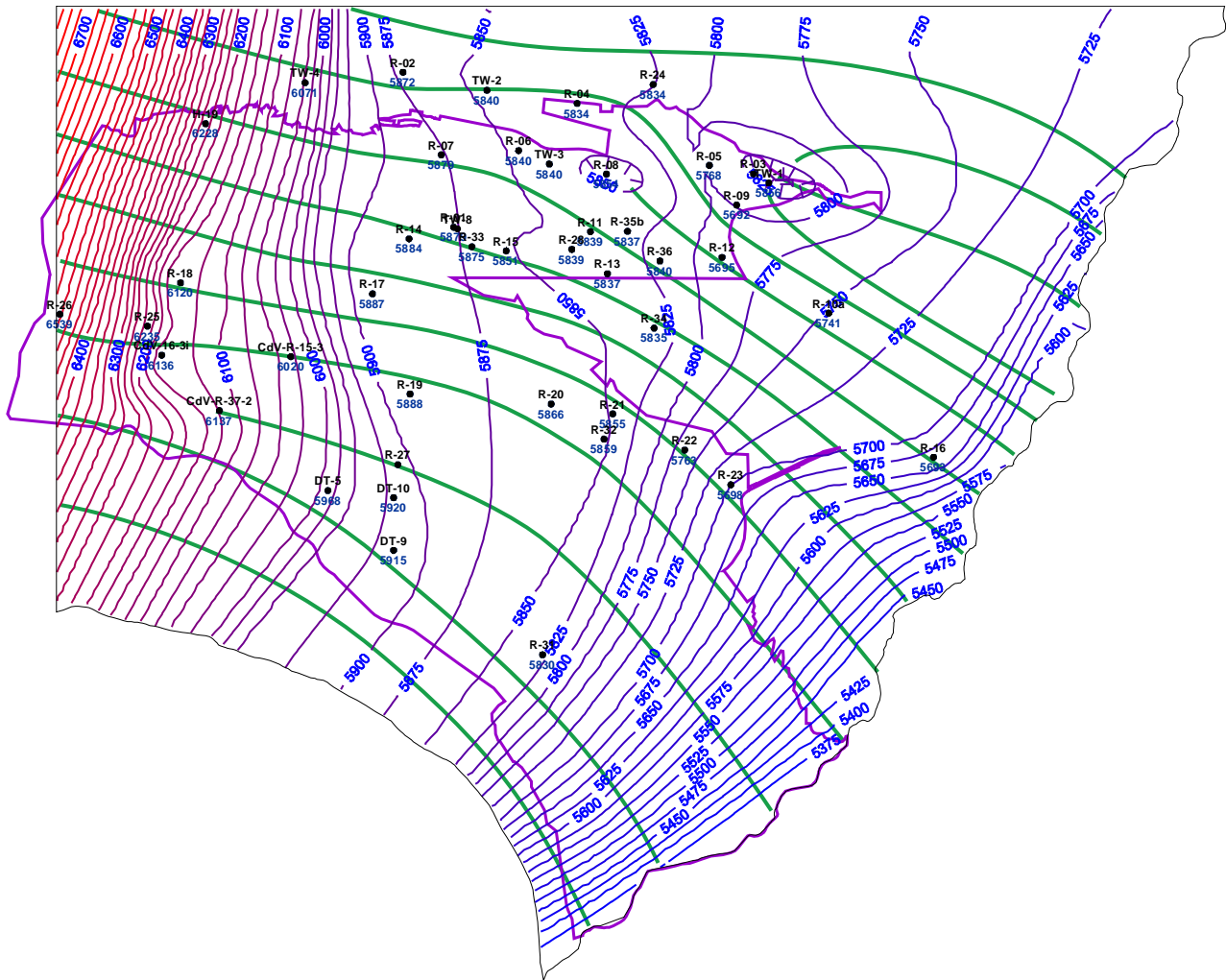
Figure H-1 Alternative water-table map 1, based on average water-table elevations in January 2006. More recent water levels observed at R-35b and R-36 are also shown.
