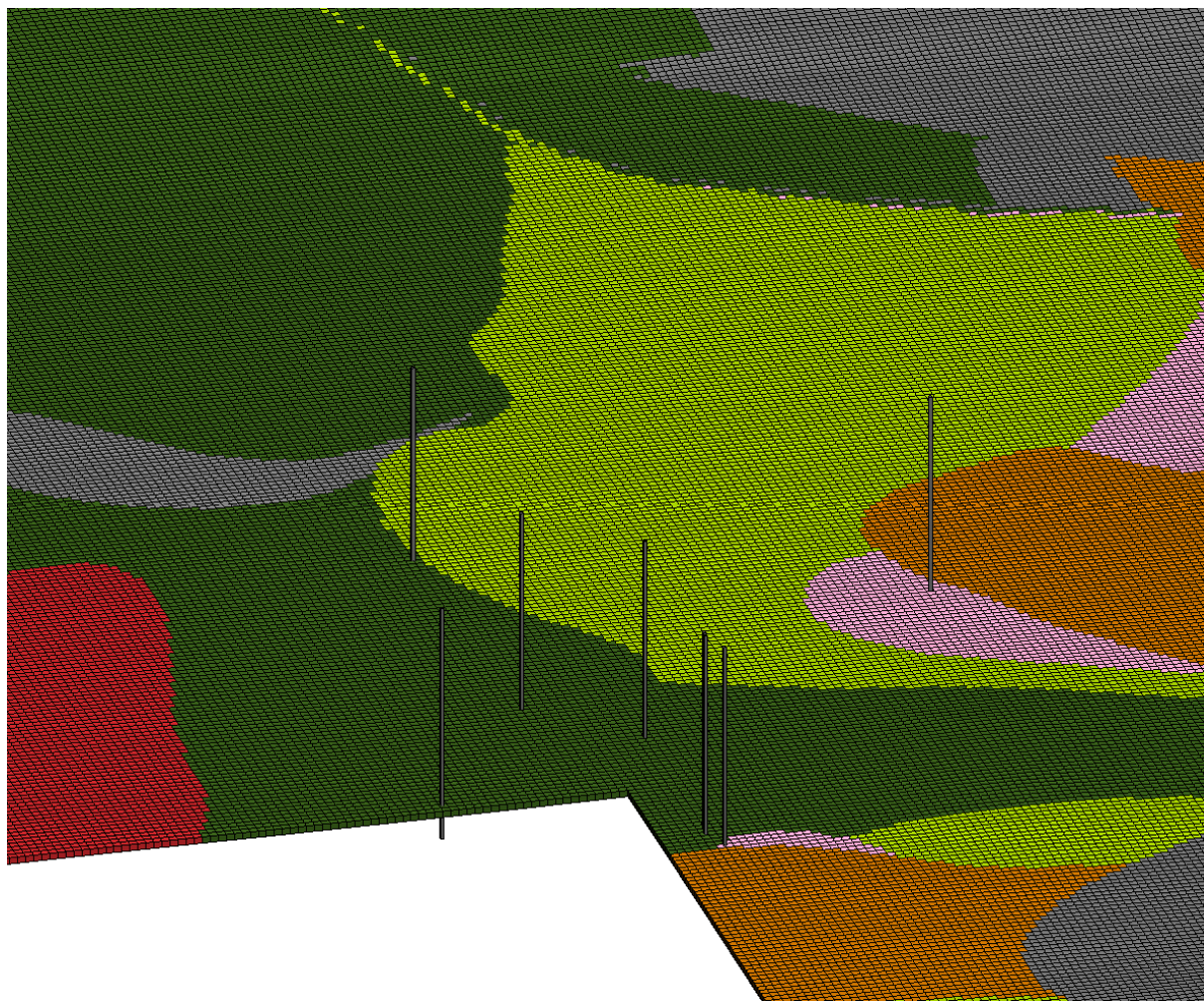
c. LGM2D cut along Sandia Canyon and well group showing 25 x 25 m uniform lateral spacing. Grid has top nodes set at elevation of the water table surface.
