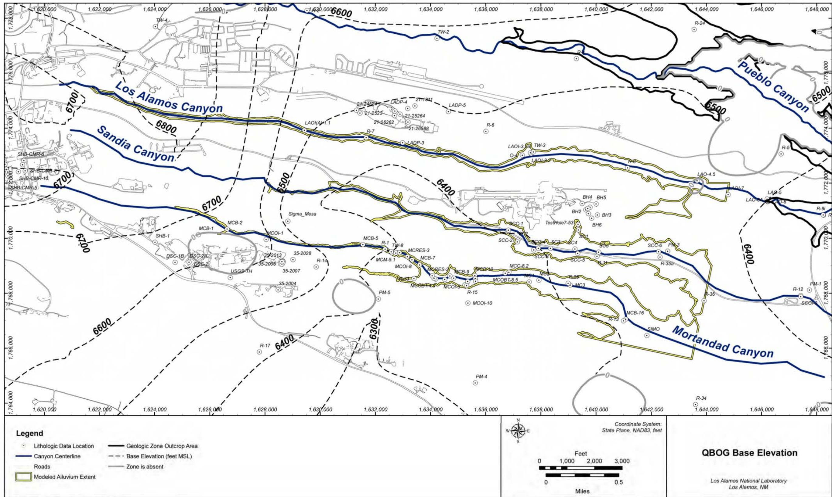
Figure J-2.0-2 Elevation contours for the base of the Guaje Pumice Bed (Qbog) in the WC08 geologic model, chromium domain. Includes outline (in yellow) defined for canyon bottom alluvium (Qa1)
