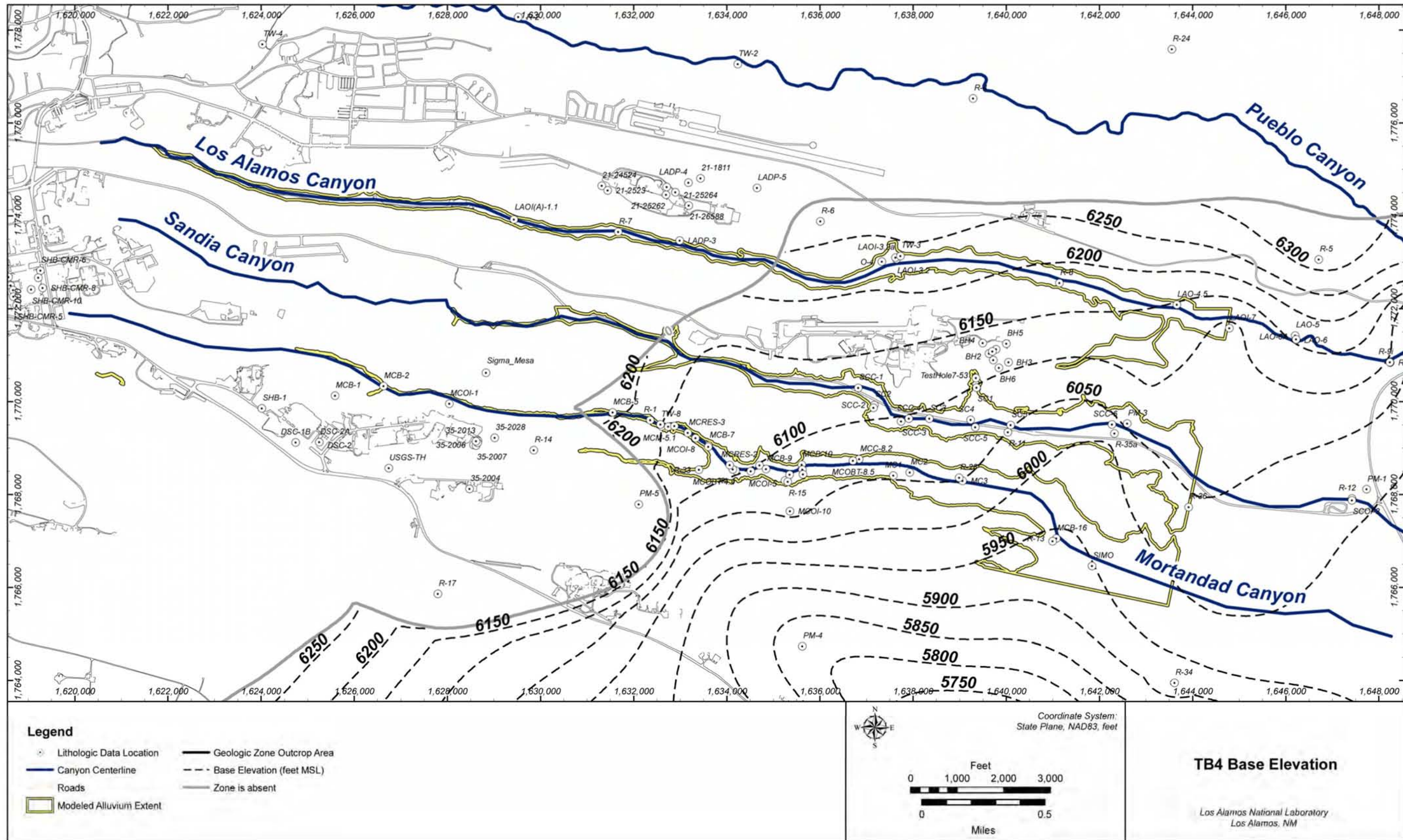
Figure J-2.0-3 Elevation contours for the base of the Cerros del Rio basalt (Tb4) in the WC08 geologic model, chromium domain
