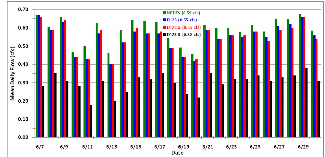
Figure C-1.0-4 Bar graphs showing mean daily flow for NPDES outfalls and gaging stations D123, D123.6, and D123.8 from June 7 to June 30, 2008, with average daily discharge shown in parentheses
