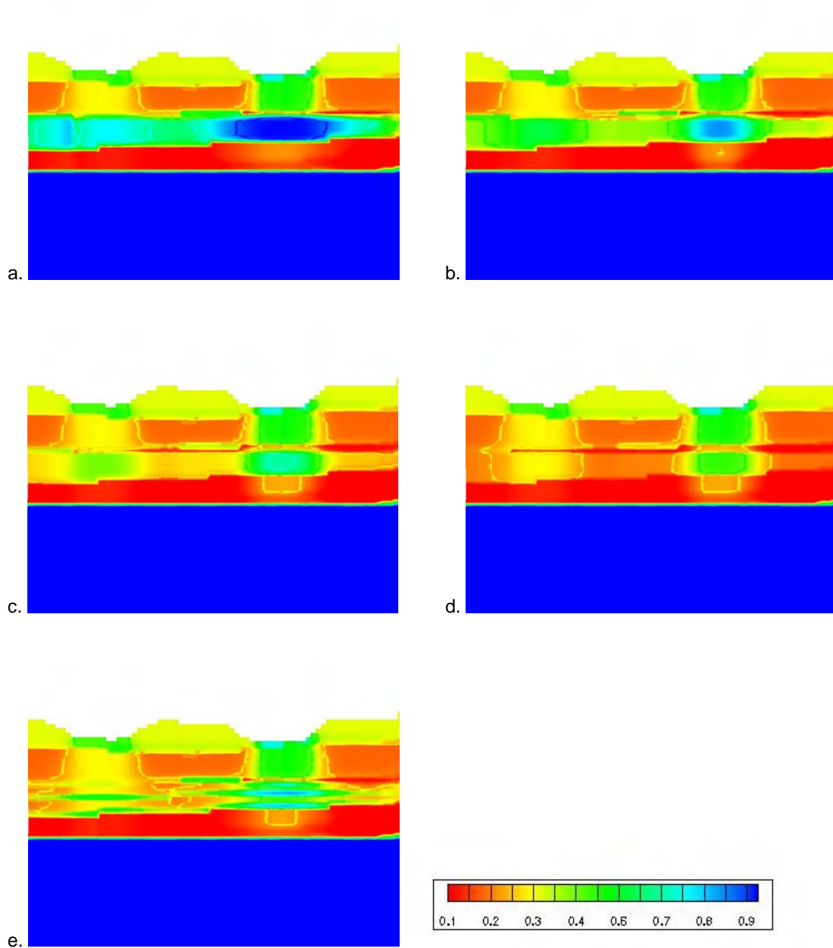
Figure J-6.3-1 Saturation profiles showing values from 0 to 1 through 3-D model (CRM) along 2-D cross-section A–A' (Figure 1.0-1) using different permeability values for the Cerros del Rio basalts : (a) 10^{-14.5} \text{ m}^2 , (b) 10^{-13.5} \text{ m}^2 , (c) 10^{-12.5} \text{ m}^2 , (d) 10^{-11.5} \text{ m}^2 , and (e) 10^{-11.5} \text{ m}^2 and permeability reduction defined for base of the Guaje Pumice Bed and base, top, and internal interface for the Cerros del Rio basalts. Sandia Canyon is the depression on the right, and Mortandad Canyon is on the left.
