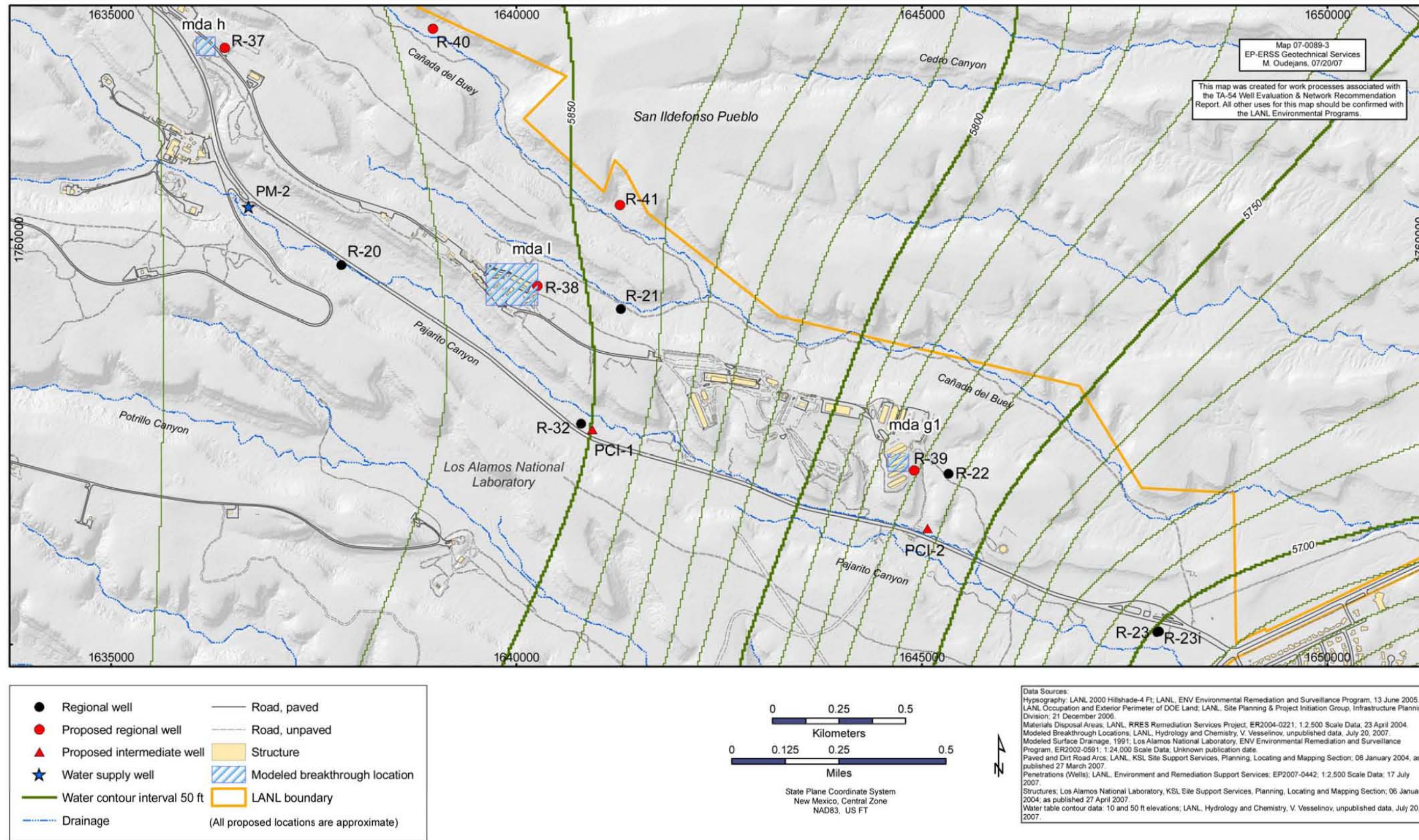
Figure C-2.0-1 Location of TA-54: MDAs H, L, and G including the existing regional wells, new proposed wells, water-table contours, water-supply wells, and the approximate breakthrough locations of mobile contaminants that have migrated through the unsaturated zone to the regional water table
