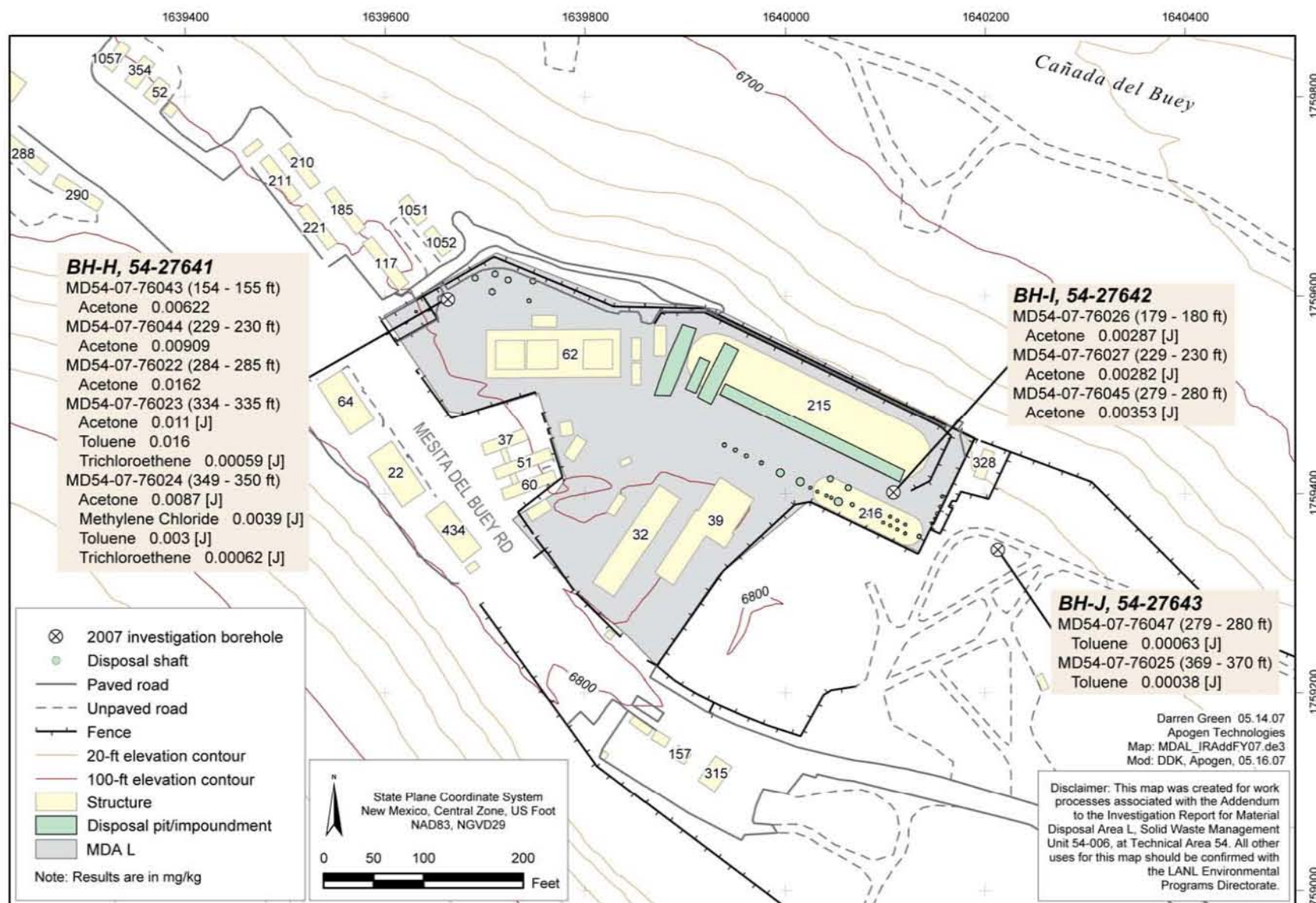
Figure 4.2-2 Supplemental investigation VOCs detected in tuff at MDA L (mg/kg)
