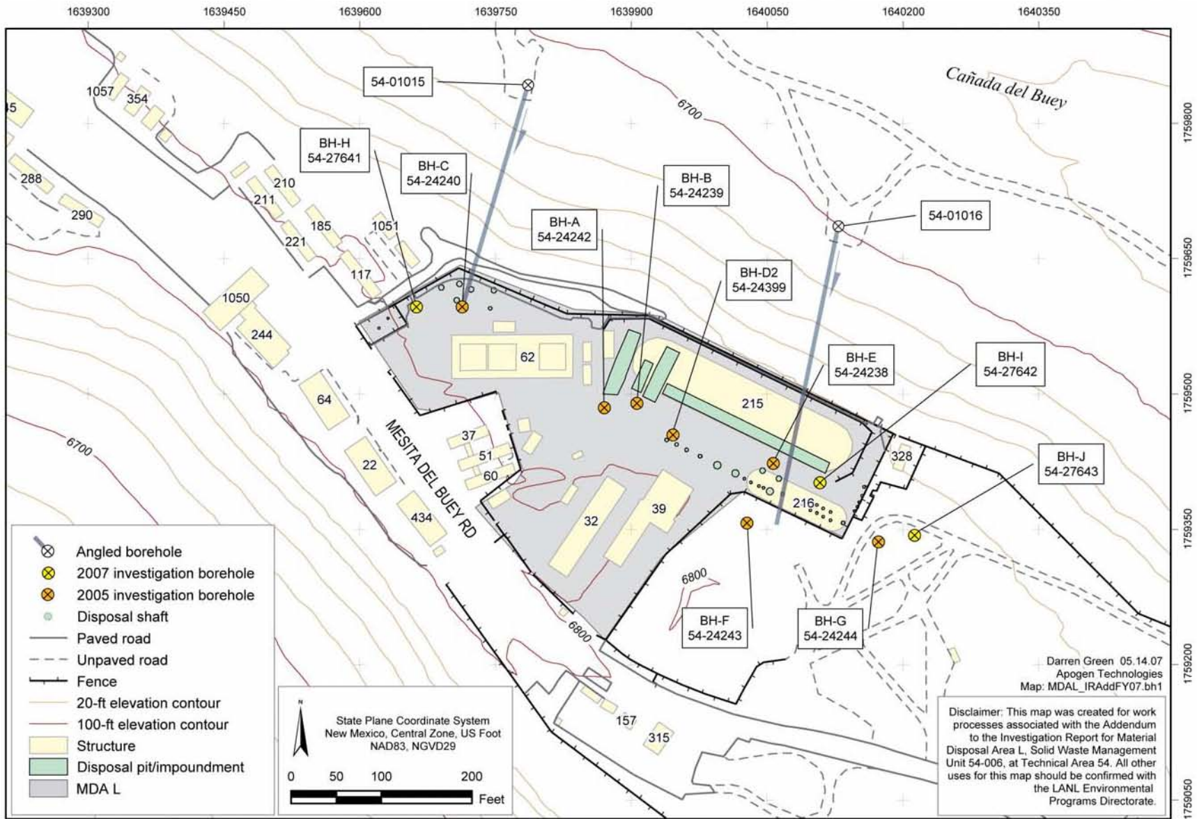
Figure 1.0-2 Locations of existing and supplemental investigation boreholes at MDA L
