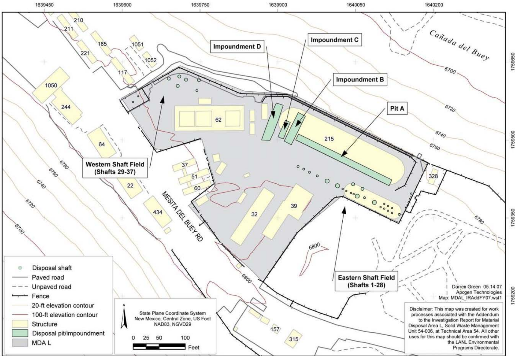
Figure 1.2-1 MDA L waste disposal units
