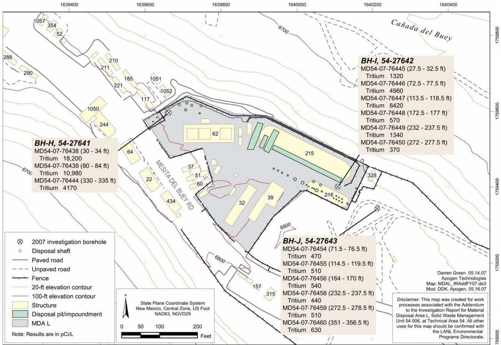
Figure 4.3-1 Supplemental investigation tritium detected in subsurface pore gas at MDA L (pCi/L)
