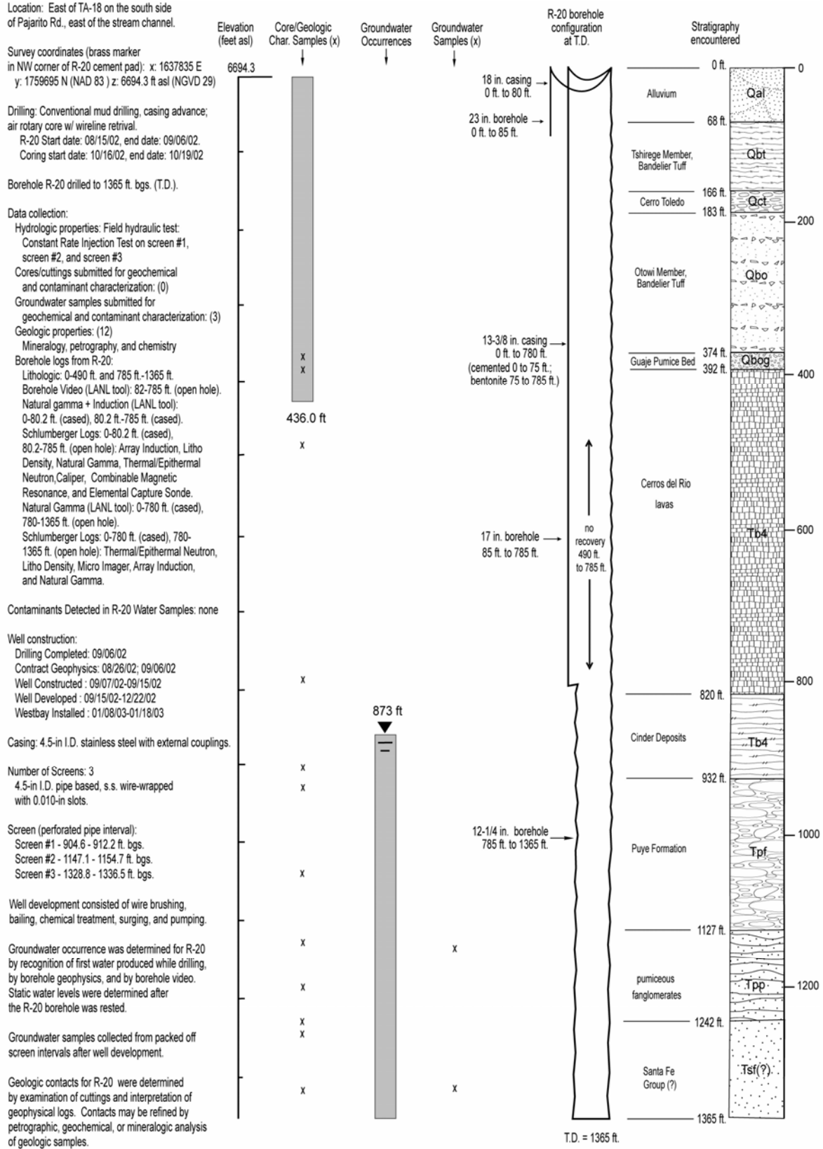
Figure 1.1-4. Summary of Well R-20 (LANL 2003, 79600)
