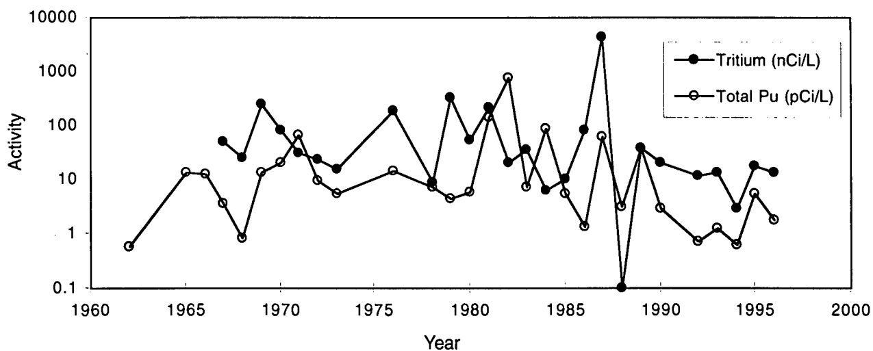
Figure 5-3. Tritium and plutonium activity at Mortandad Canyon at Gaging Station 1.
