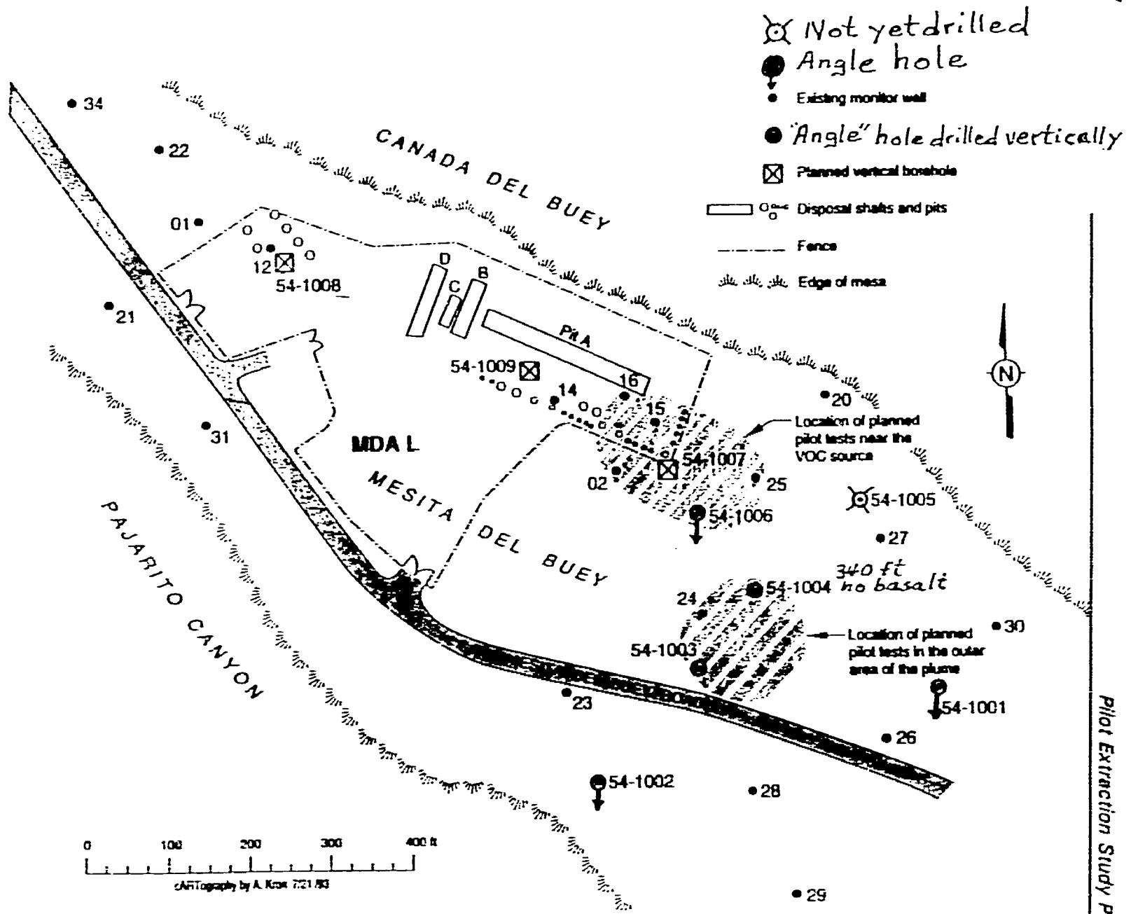
Location map of planned boreholes and pilot tests
