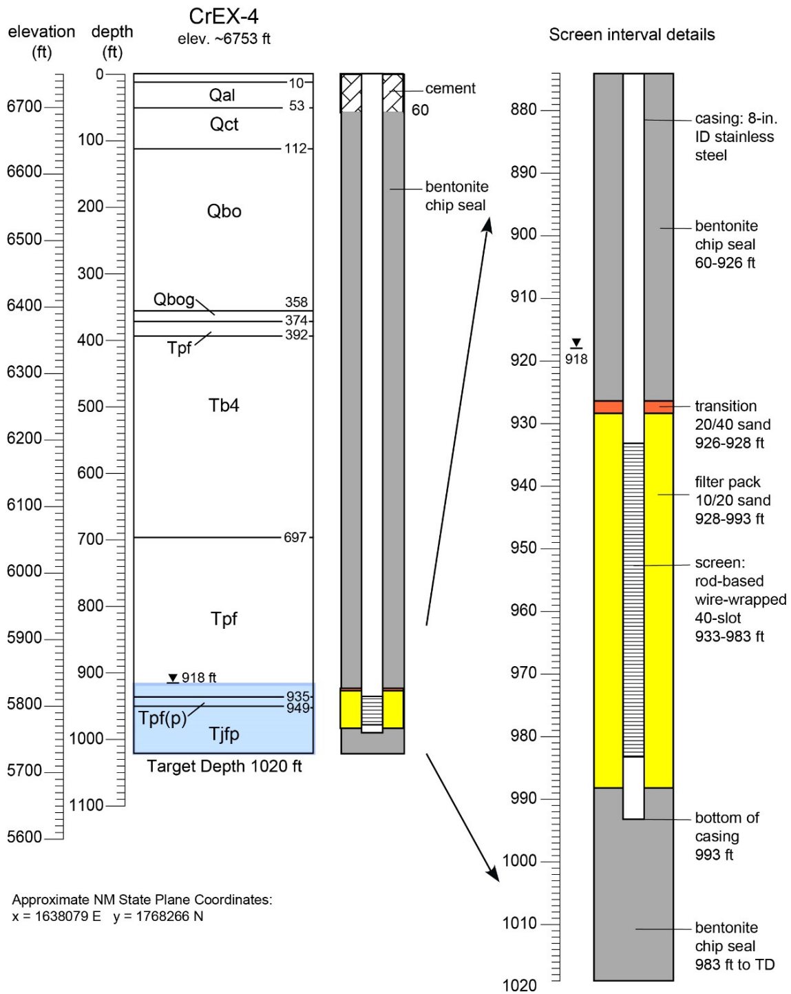
Figure 2 Predicted geology and preliminary well design for well CrEX-4
