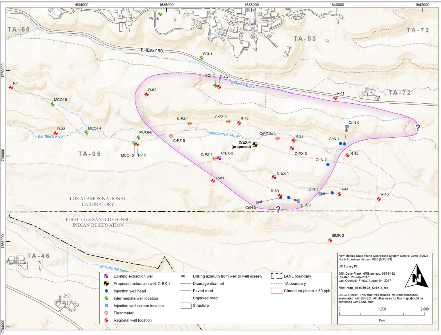
Figure 1 Proposed location for extraction well CrEX-4
