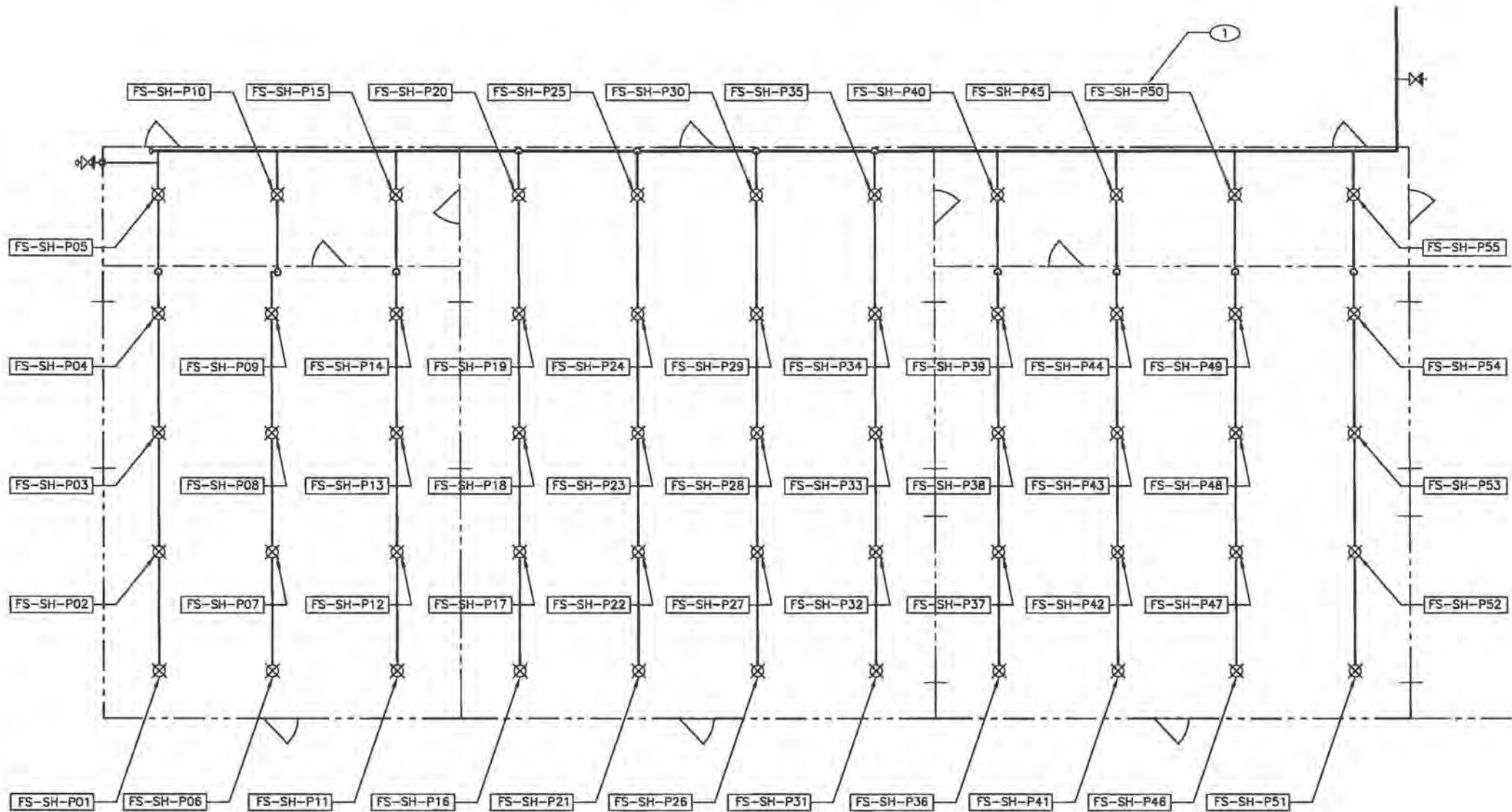
PERMACON SPRINKLER HEADS LOCATION PLAN SCALE: NONE
