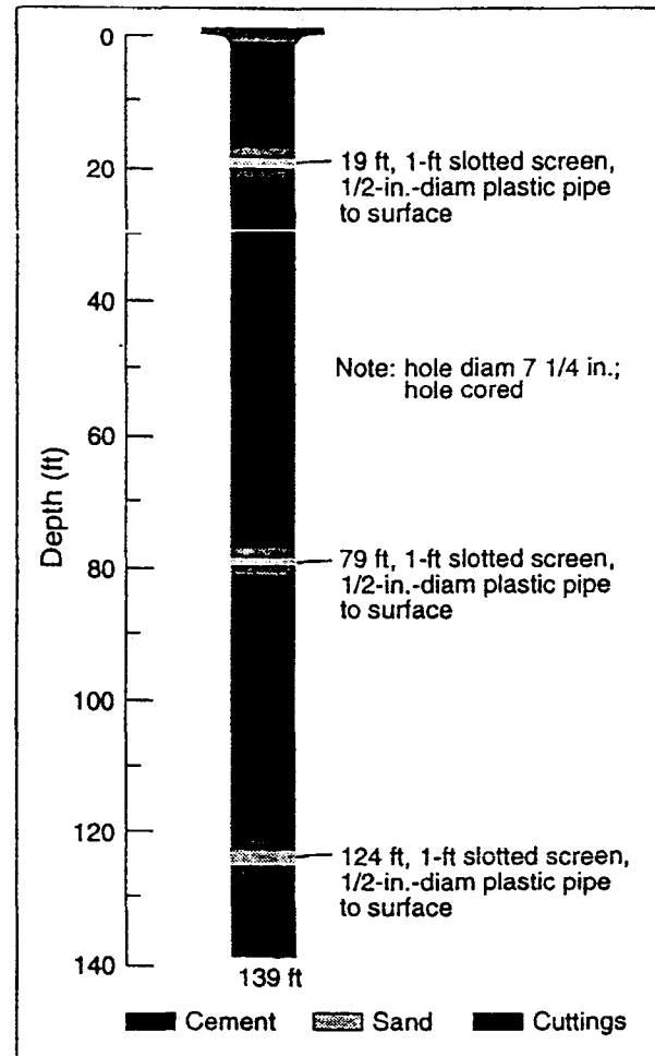
Figure VII-6b. Test hole TBM-1 constructed with three zones to measure barometric pressures in the tuff at depths of 19, 79, and 124 ft.
