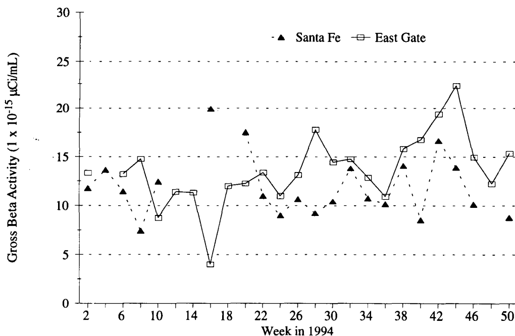
Figure V-9. Gross beta activity in air at one regional and one perimeter location.
