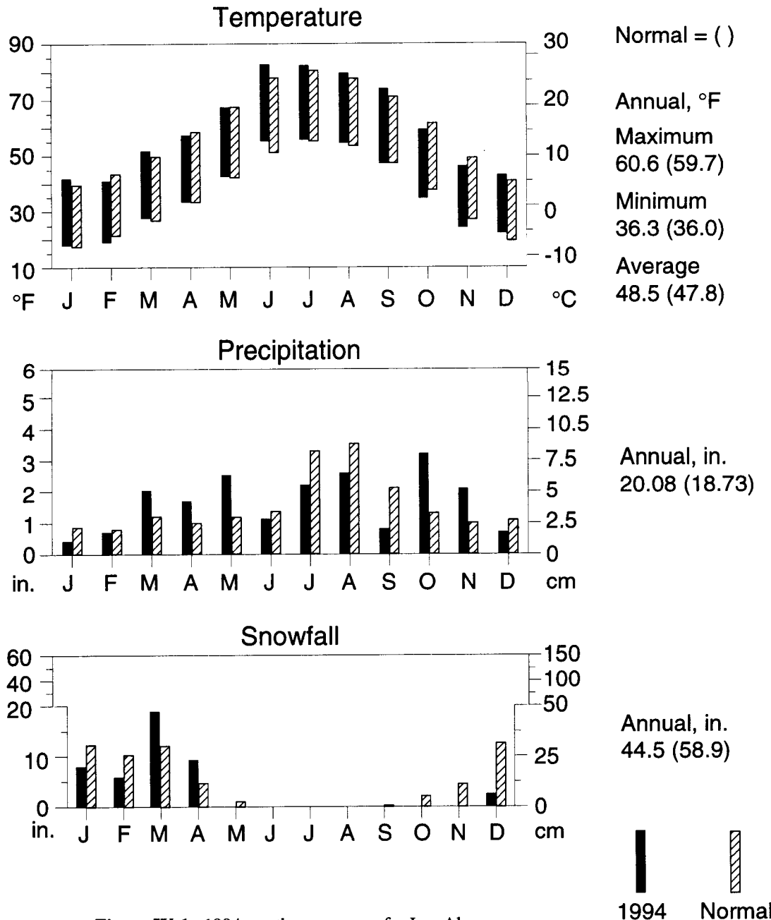
Figure IV-1. 1994 weather summary for Los Alamos.
