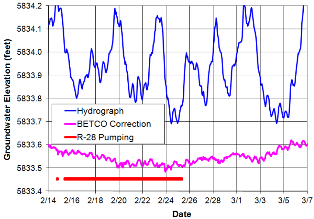
Well R-13 hydrograph
