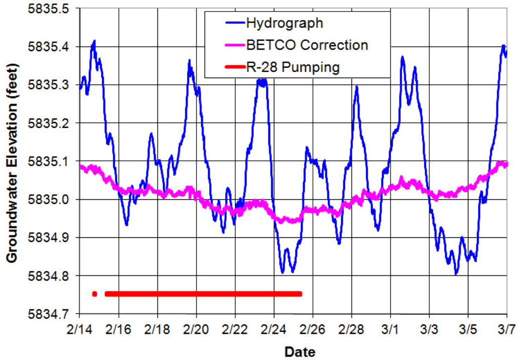
Well R-44 screen 1 hydrograph
