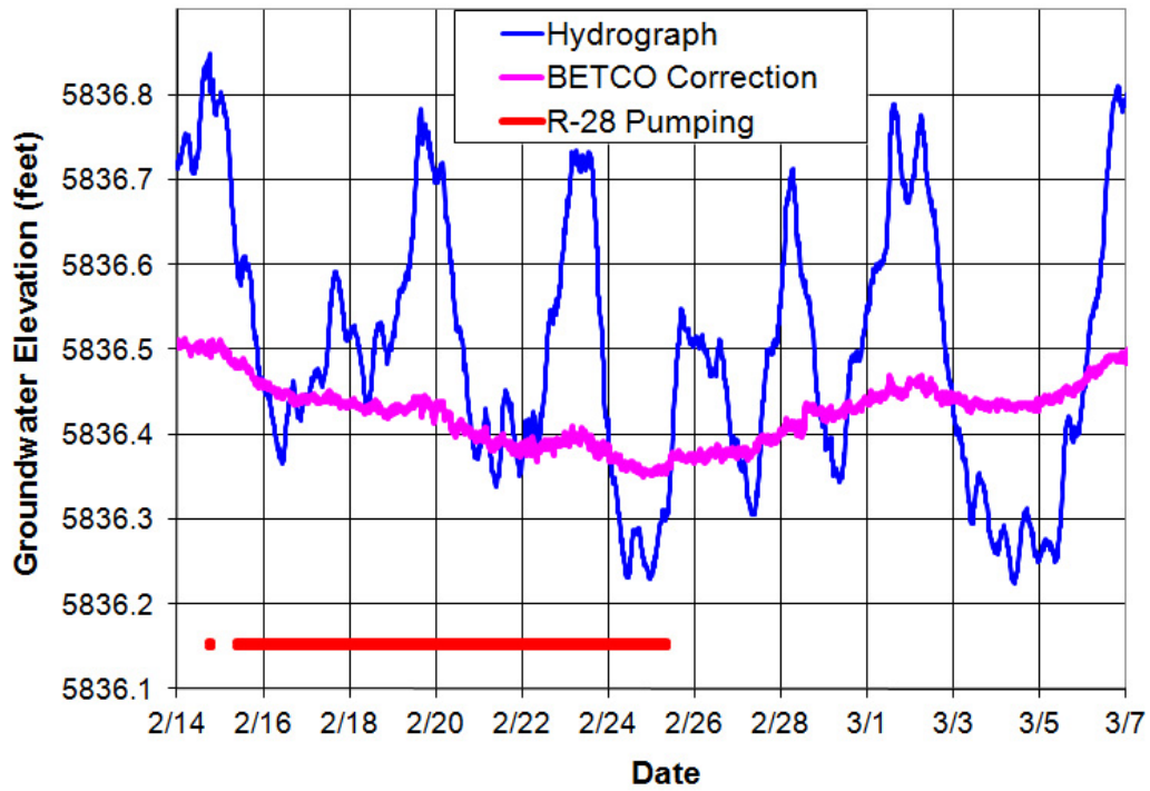
Well R-50 screen 1 hydrograph
