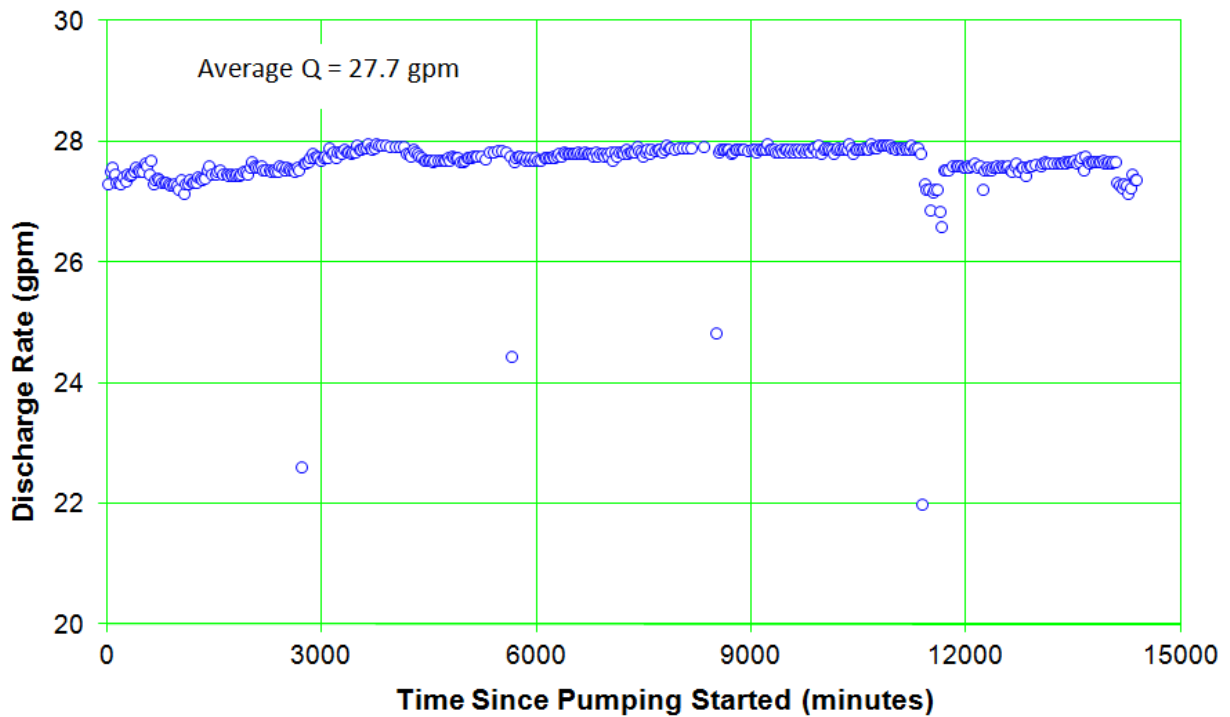
Well R-28 measured pumping rate
