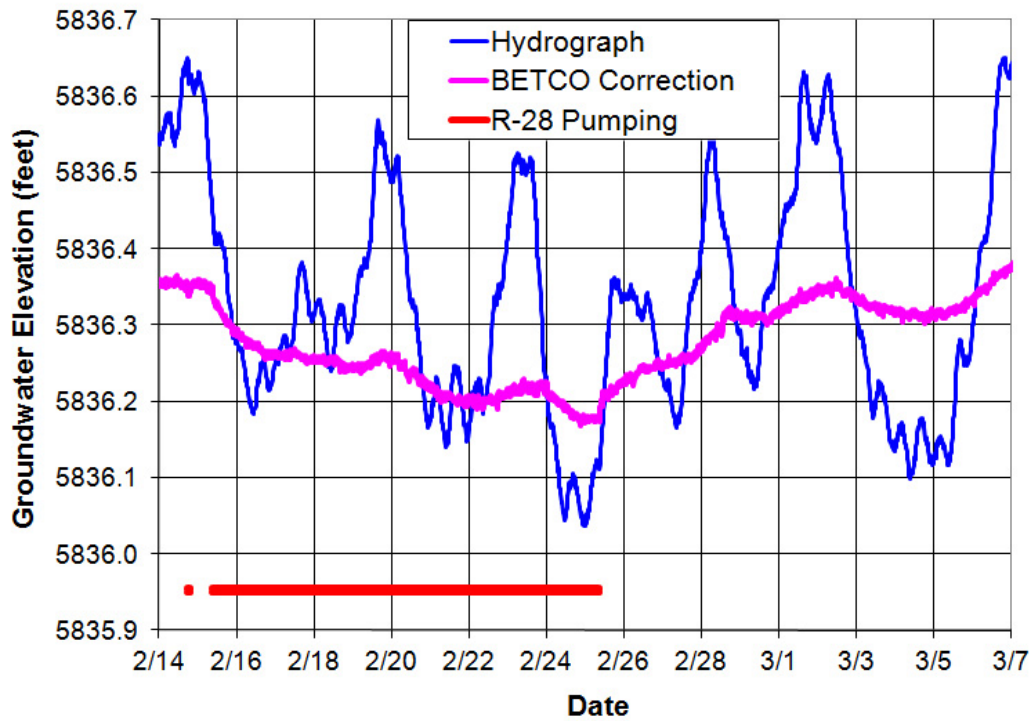
Well R-50 screen 2 hydrograph
