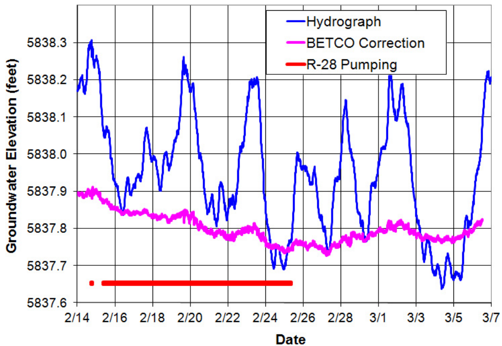
Well R-42 hydrograph
