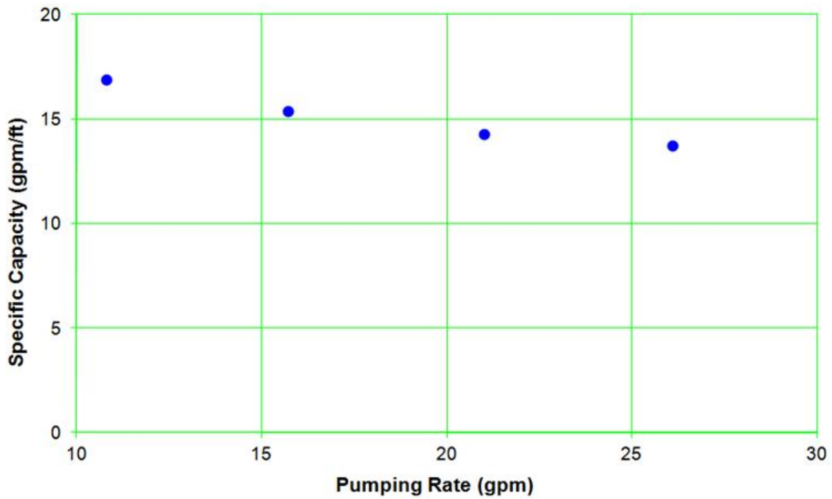
Well R-28 specific capacity
