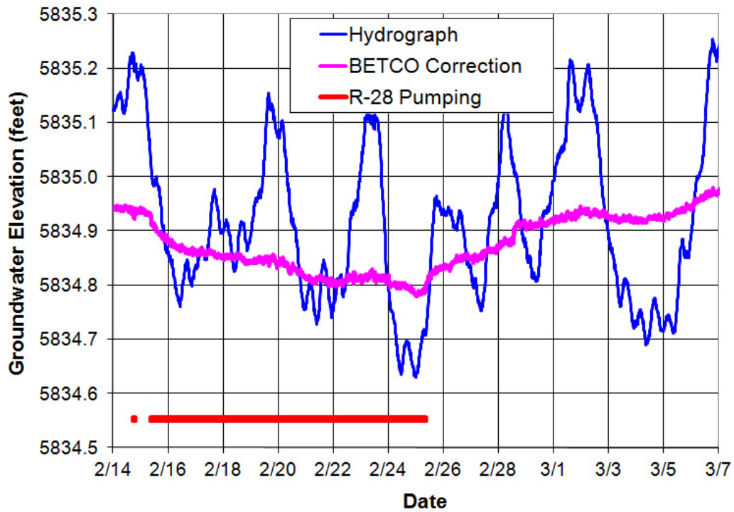
Well R-44 screen 2 hydrograph
