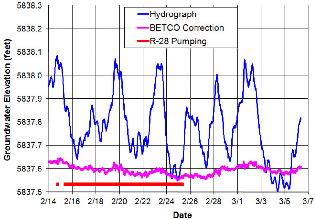
Well R-43 screen 1 hydrograph
