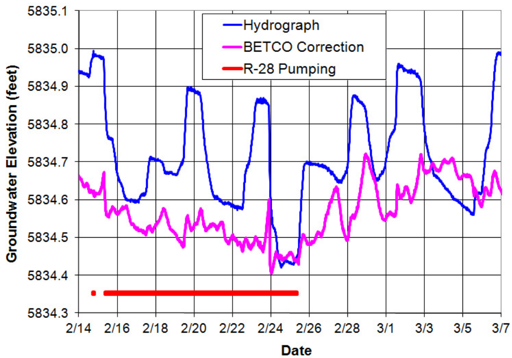
Well R-45 screen 2 hydrograph
