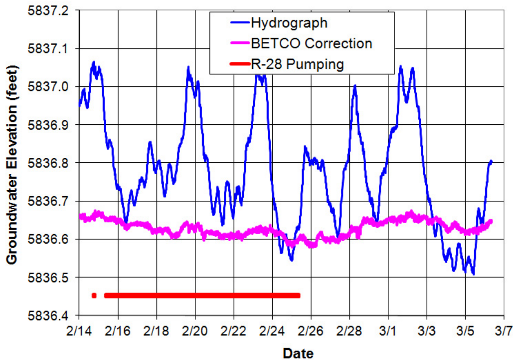
Well R-43 screen 2 hydrograph
