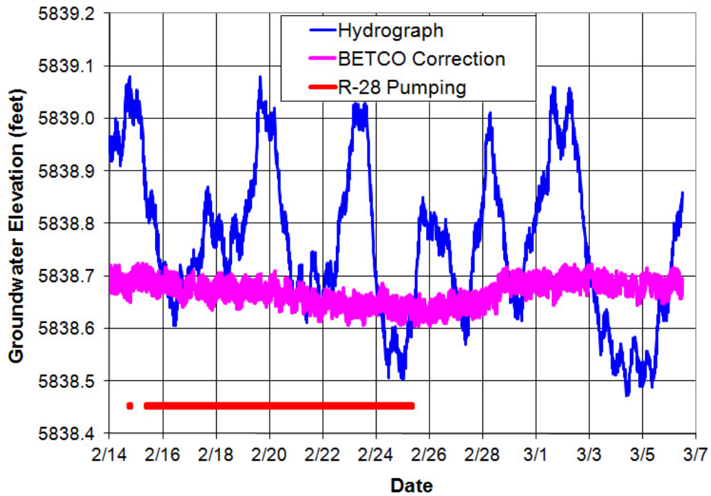
Well R-61 screen 2 hydrograph
