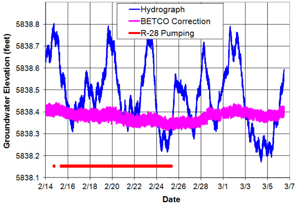
Well R-61 screen 1 hydrograph
