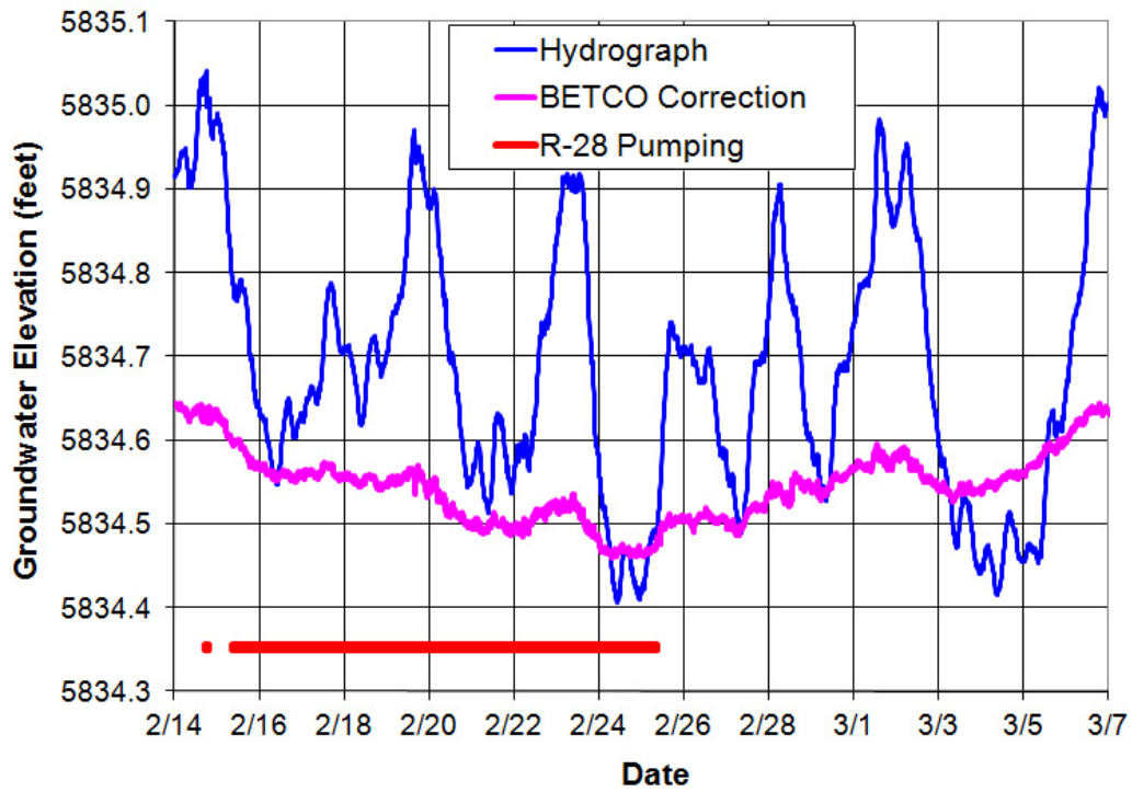
Well R-45 screen 1 hydrograph
