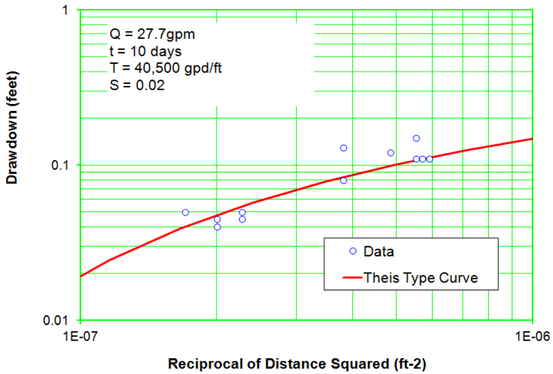
Well R-28 distance-drawdown at 10 days
