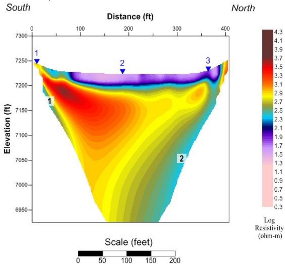
Figure 8. Profile 5 Model Resistivity Results - Identifying Electrical Resistivity Features of Interest, includes Visual Aids of Potential Structural Features.
