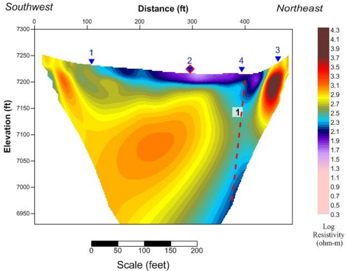
Figure 9. Profile 6 Model Resistivity Results - Identifying Electrical Resistivity Features of Interest, includes Visual Aids of Potential Structural Features.
