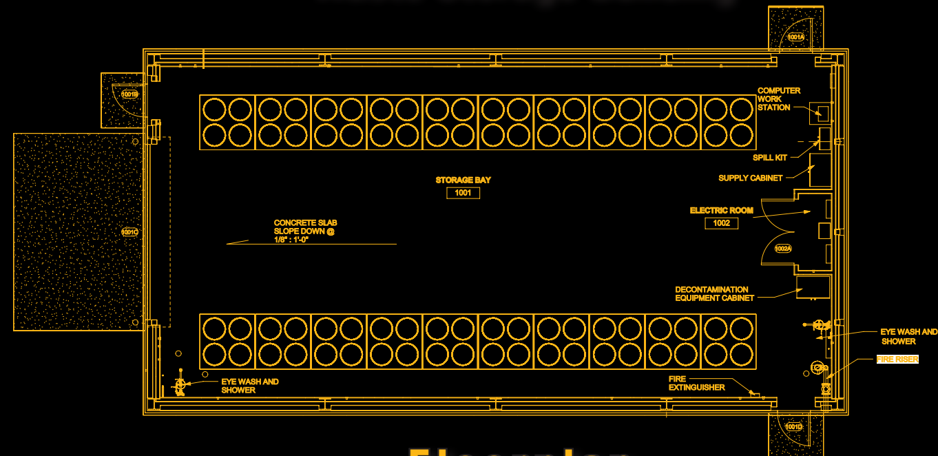
Floorplan
