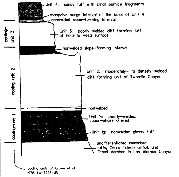
SCHMATIC STRATIGRAPHY OF THE TSHIREGE MEMBER IN THE TA-55 AREA
