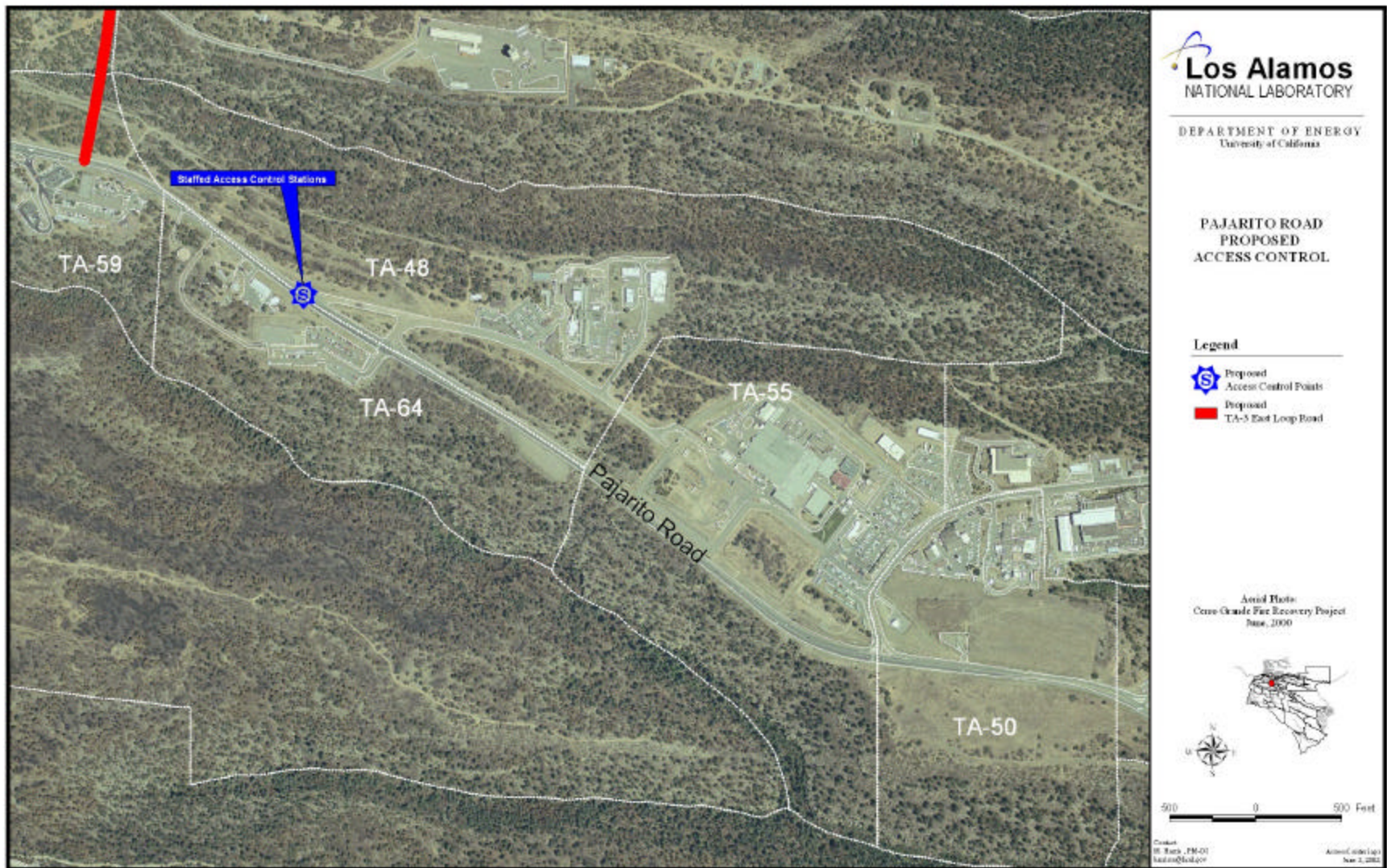
Figure 3. Proposed Pajarito Road access controls.
